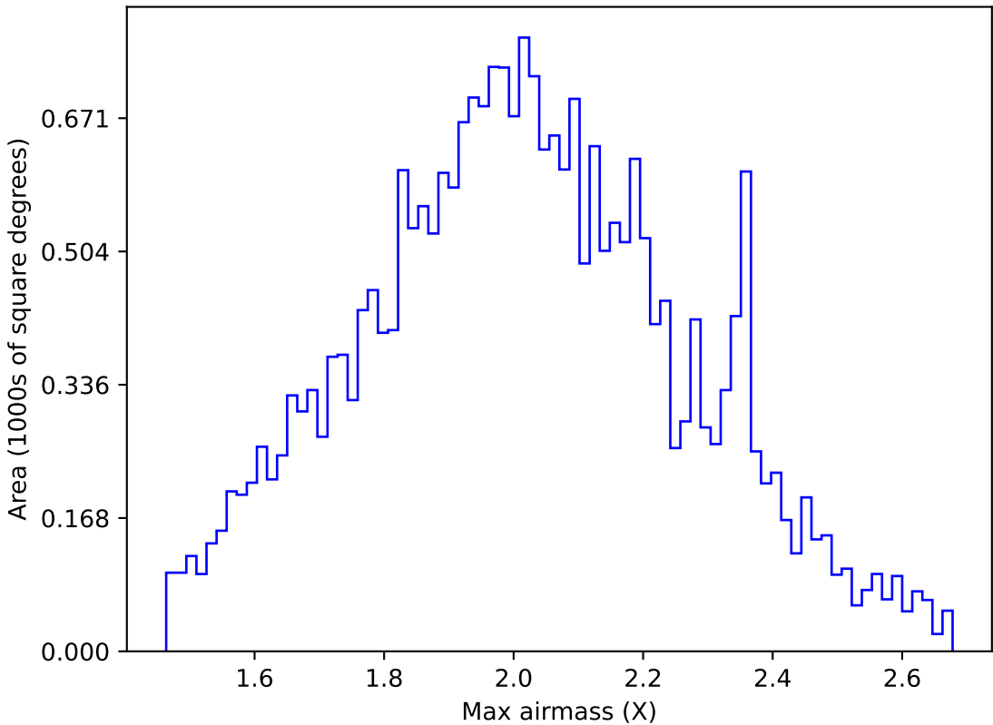
too_elab_r16_d3_gz_v3.4_10yrs All sky g band: Max airmass
