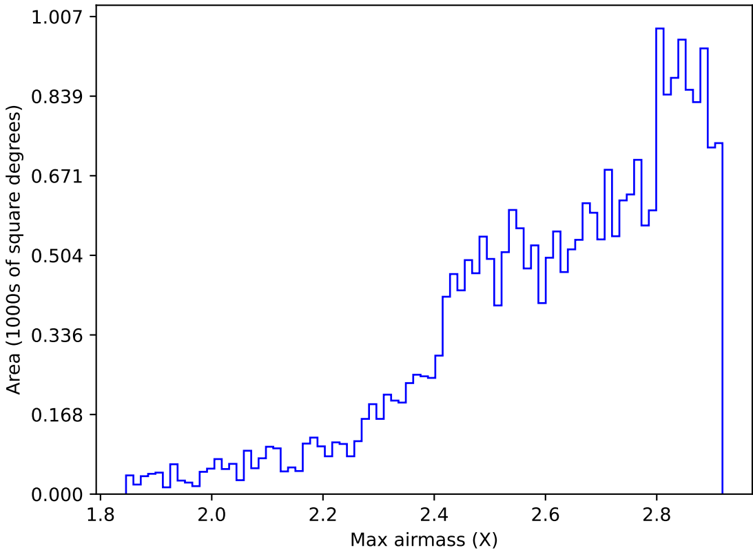
too_elab_r16_d3_gz_v3.4_10yrs All sky all bands: Max airmass
