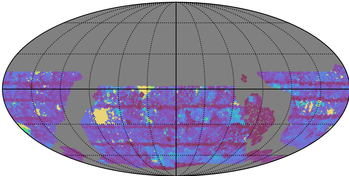
too_elab_r16_d3_gz_v3.4_10yrs WFD z band: Max Inter-Night Gap
