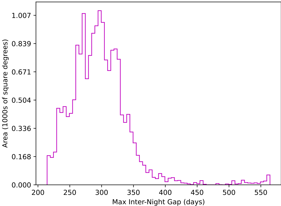
too_elab_r16_d3_gz_v3.4_10yrs WFD z band: Max Inter-Night Gap
