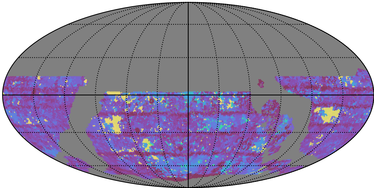
too_elab_r16_d3_gz_v3.4_10yrs WFD y band: Max Inter-Night Gap
