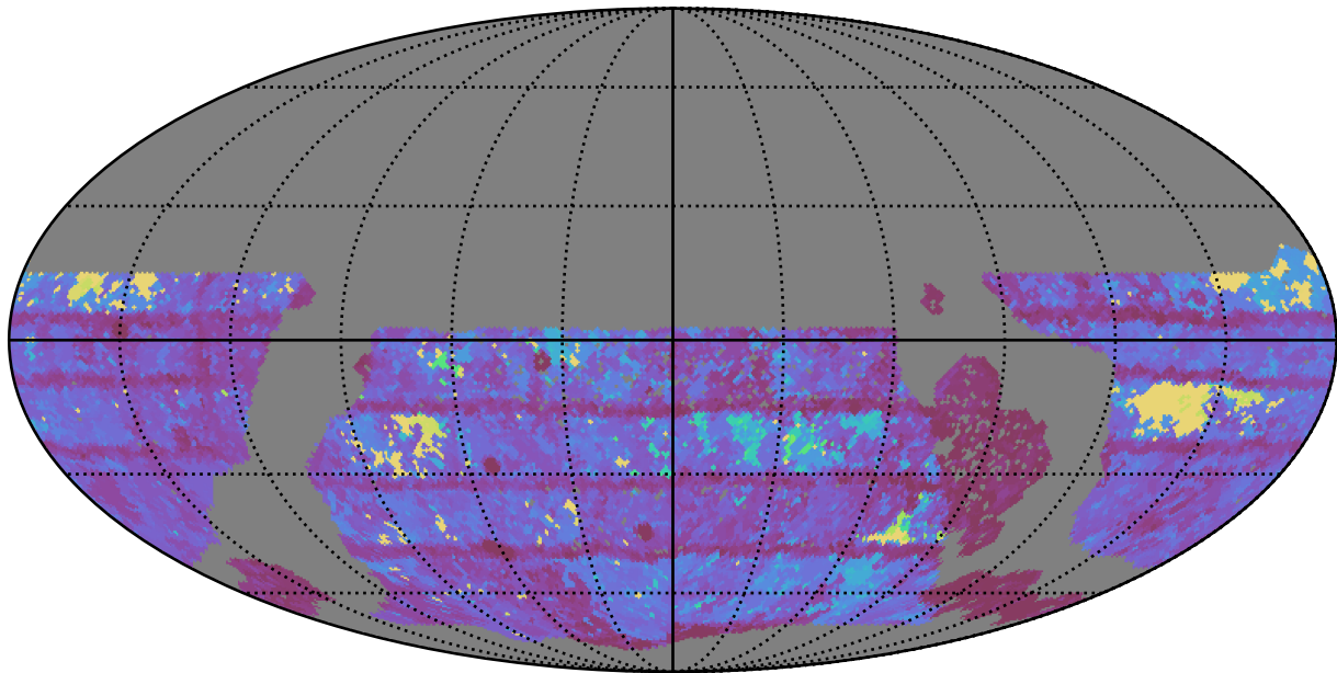
too_elab_r16_d3_gz_v3.4_10yrs WFD r band: Max Inter-Night Gap
