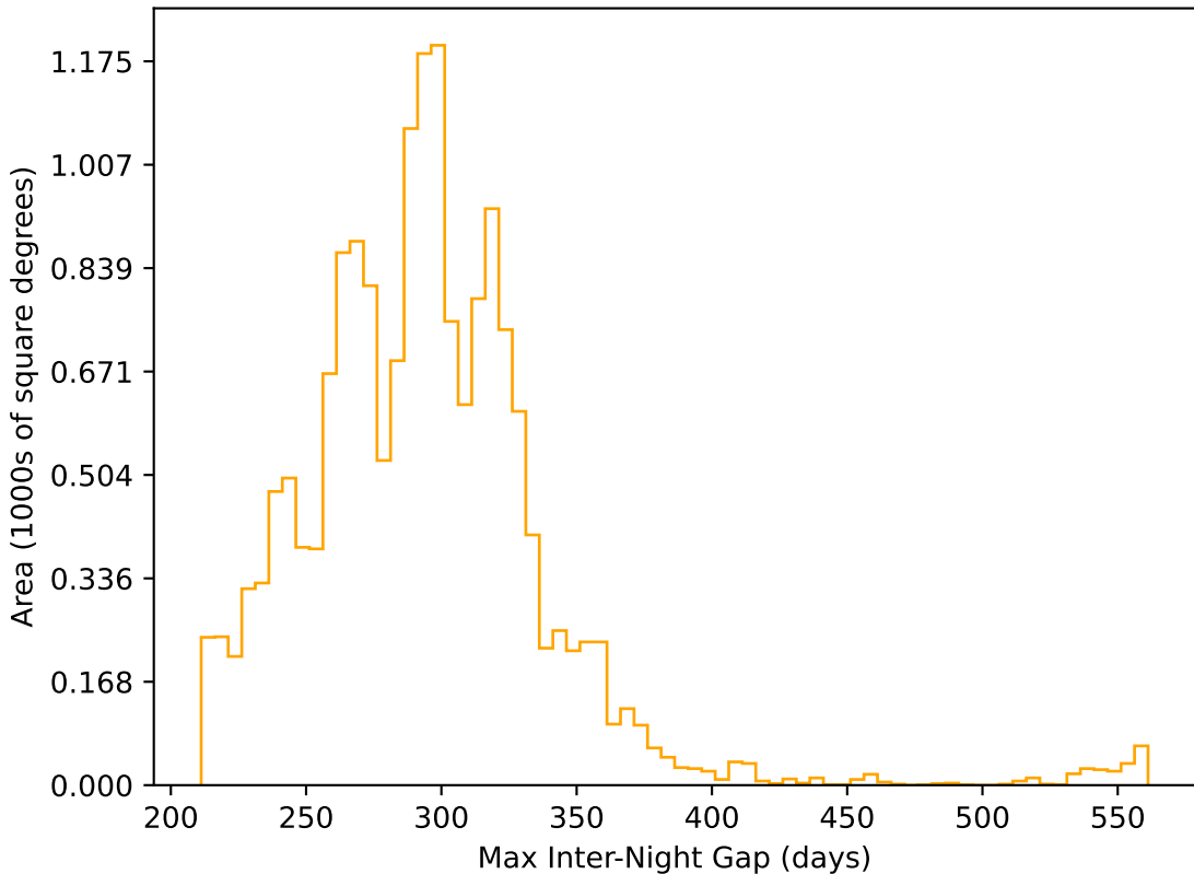
too_elab_r16_d3_gz_v3.4_10yrs WFD r band: Max Inter-Night Gap
