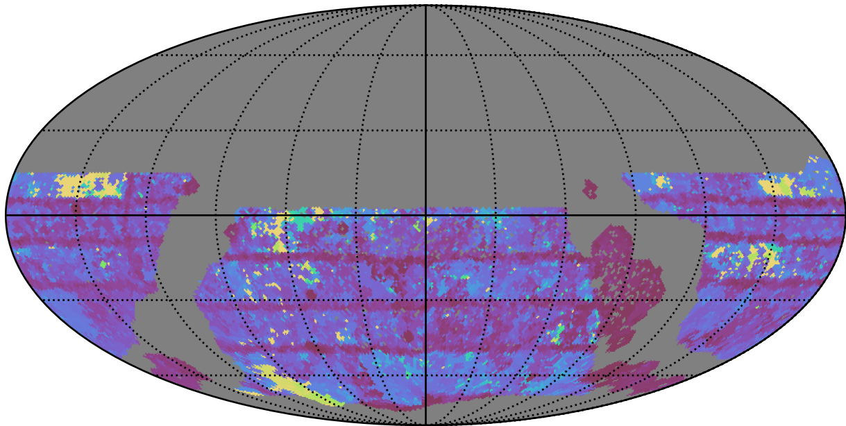
too_elab_r16_d3_gz_v3.4_10yrs WFD i band: Max Inter-Night Gap
