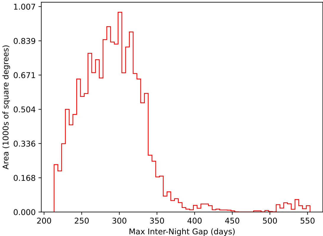
too_elab_r16_d3_gz_v3.4_10yrs WFD i band: Max Inter-Night Gap
