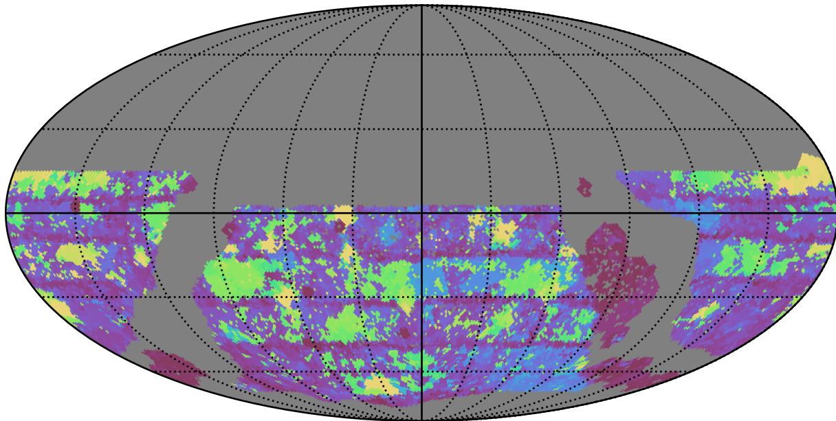
too_elab_r16_d3_gz_v3.4_10yrs WFD g band: Max Inter-Night Gap
