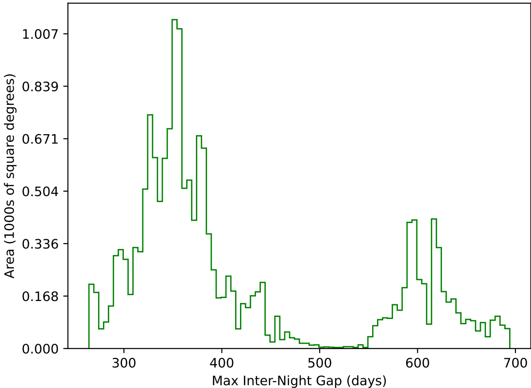
too_elab_r16_d3_gz_v3.4_10yrs WFD g band: Max Inter-Night Gap
