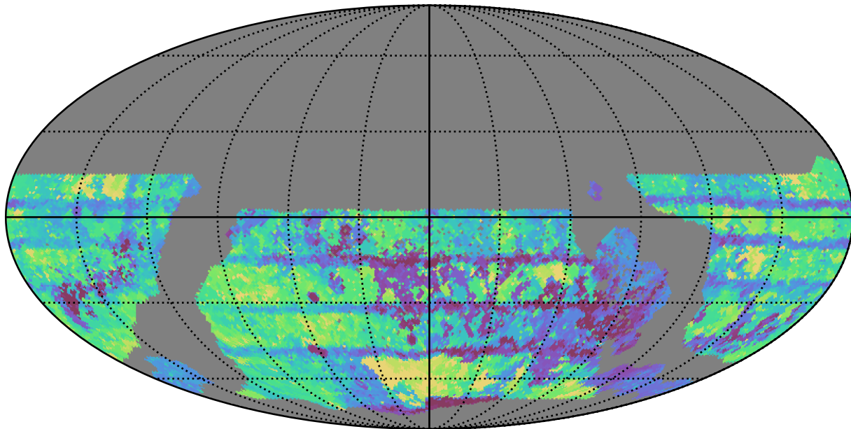
too_elab_r16_d3_gz_v3.4_10yrs WFD all bands: Max Inter-Night Gap
