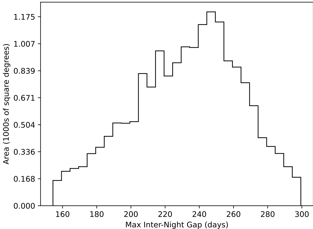
too_elab_r16_d3_gz_v3.4_10yrs WFD all bands: Max Inter-Night Gap
