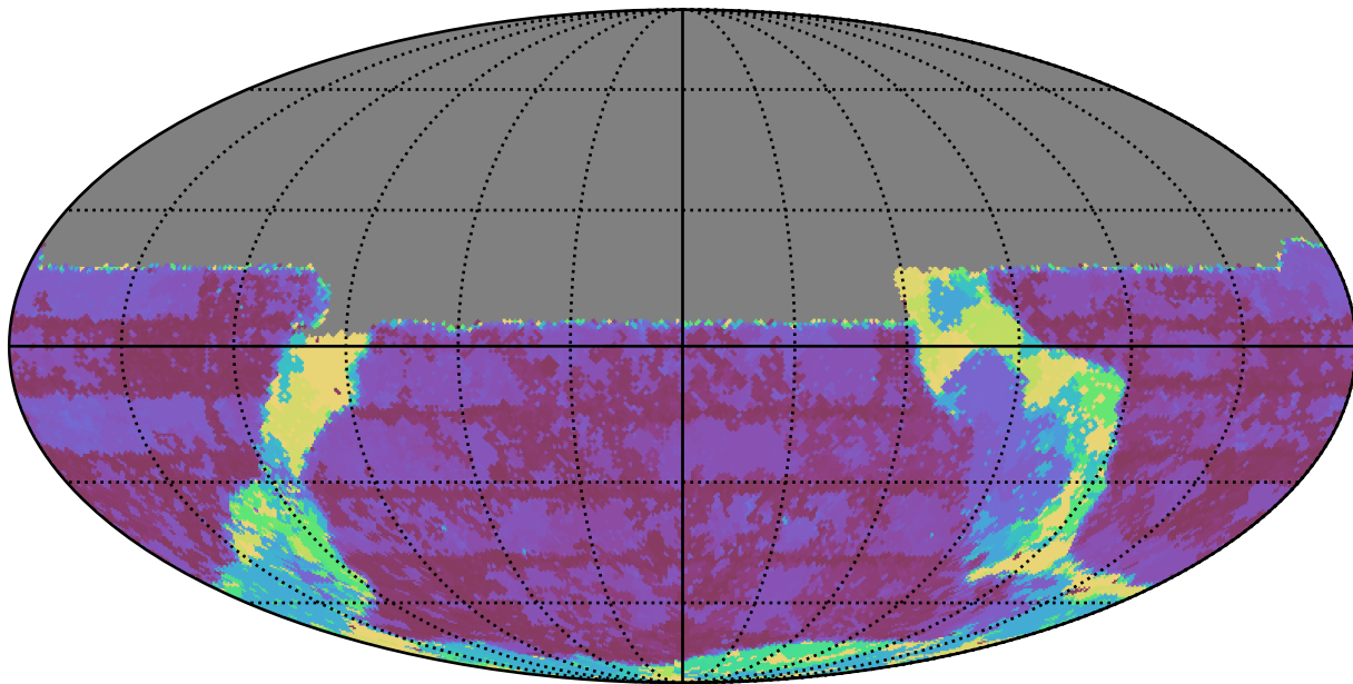
too_elab_r16_d3_gz_v3.4_10yrs All sky u band: Max Inter-Night Gap
