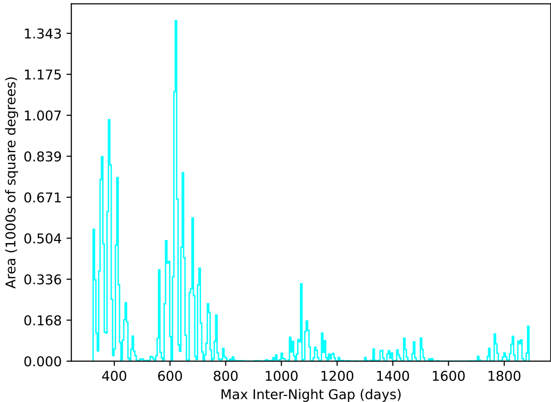
too_elab_r16_d3_gz_v3.4_10yrs All sky u band: Max Inter-Night Gap
