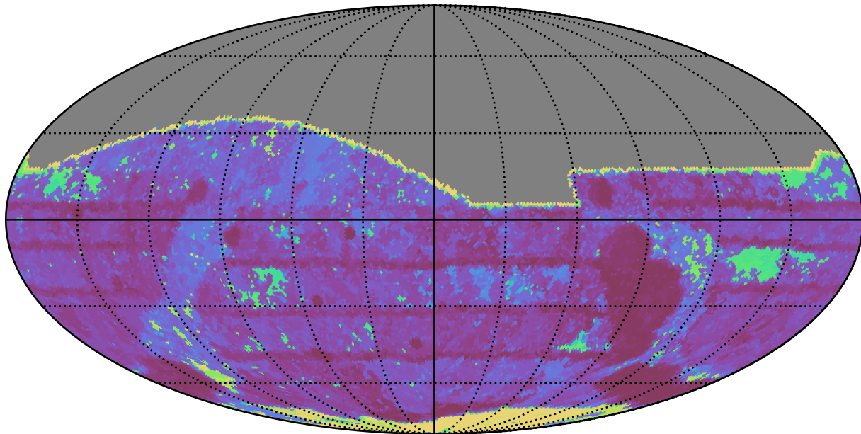
too_elab_r16_d3_gz_v3.4_10yrs All sky r band: Max Inter-Night Gap
