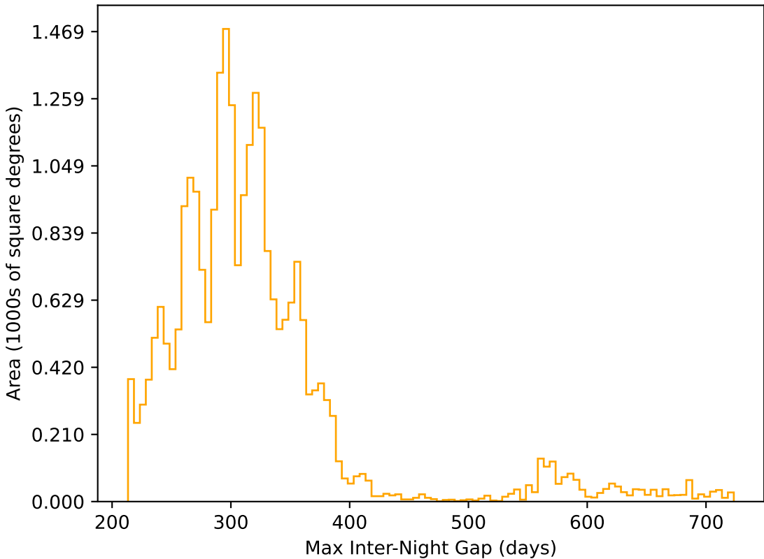
too_elab_r16_d3_gz_v3.4_10yrs All sky r band: Max Inter-Night Gap
