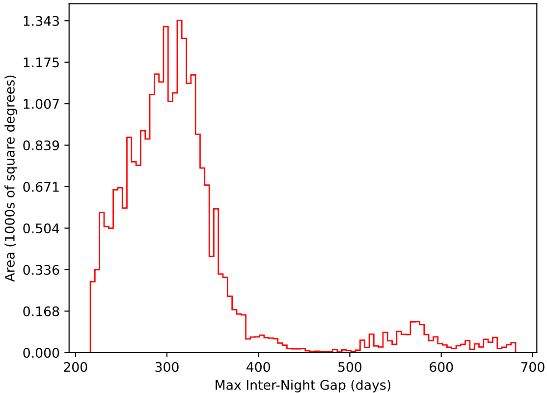
too_elab_r16_d3_gz_v3.4_10yrs All sky i band: Max Inter-Night Gap
