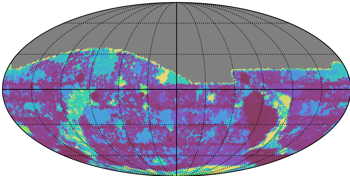
too_elab_r16_d3_gz_v3.4_10yrs All sky g band: Max Inter-Night Gap
