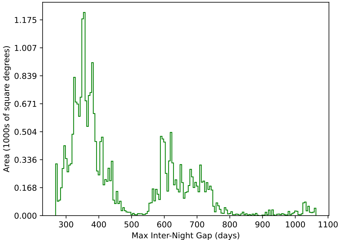
too_elab_r16_d3_gz_v3.4_10yrs All sky g band: Max Inter-Night Gap
