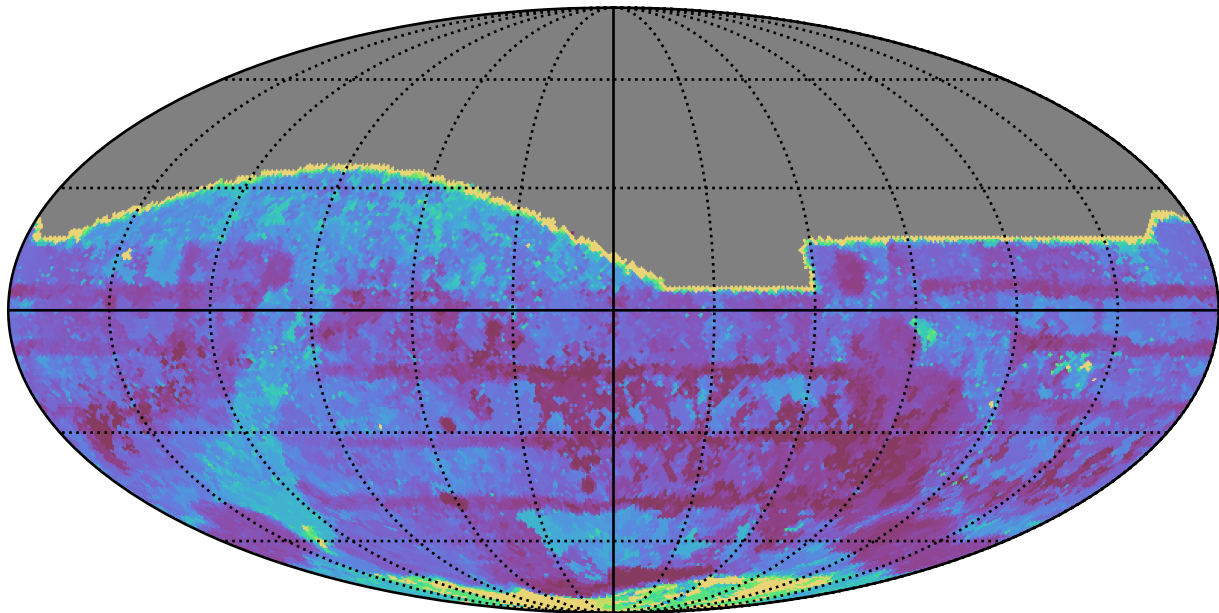
too_elab_r16_d3_gz_v3.4_10yrs All sky all bands: Max Inter-Night Gap
