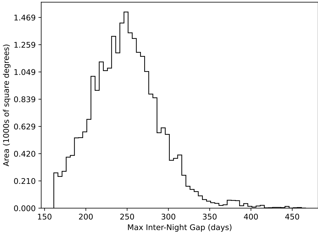
too_elab_r16_d3_gz_v3.4_10yrs All sky all bands: Max Inter-Night Gap
