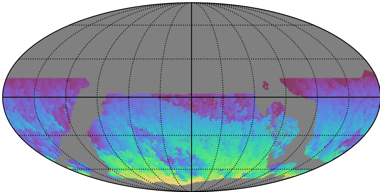
too_elab_r16_d3_gz_v3.4_10yrs WFD z band: Max HA
