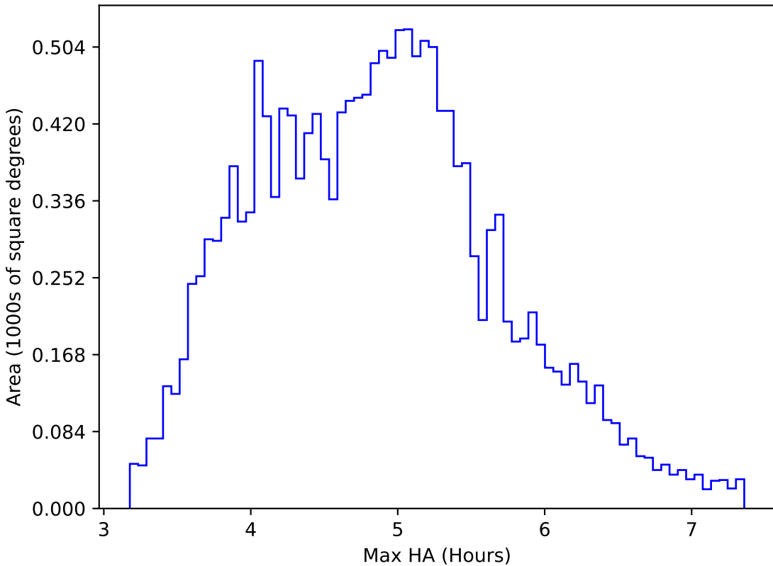
too_elab_r16_d3_gz_v3.4_10yrs WFD z band: Max HA
