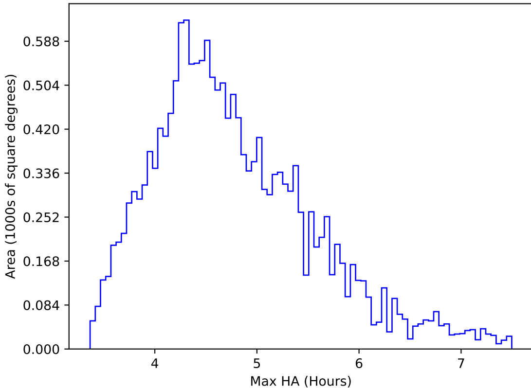
too_elab_r16_d3_gz_v3.4_10yrs WFD y band: Max HA
