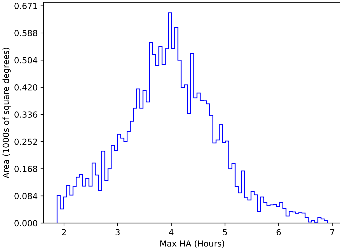
too_elab_r16_d3_gz_v3.4_10yrs WFD u band: Max HA
