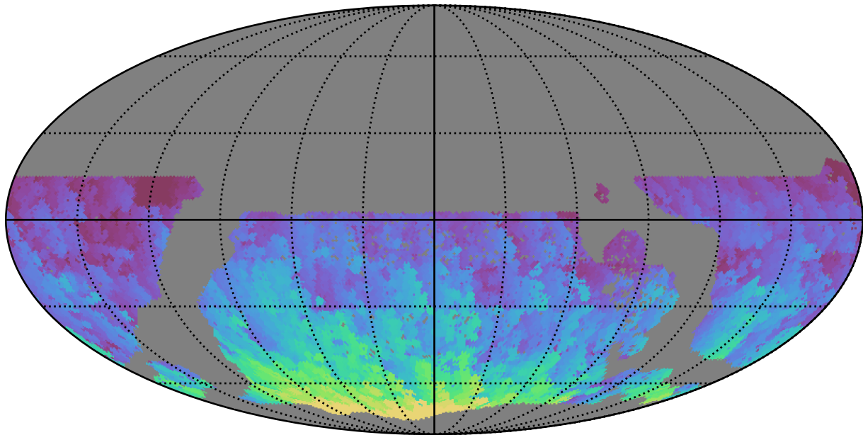
too_elab_r16_d3_gz_v3.4_10yrs WFD r band: Max HA
