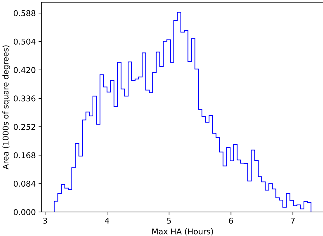
too_elab_r16_d3_gz_v3.4_10yrs WFD i band: Max HA
