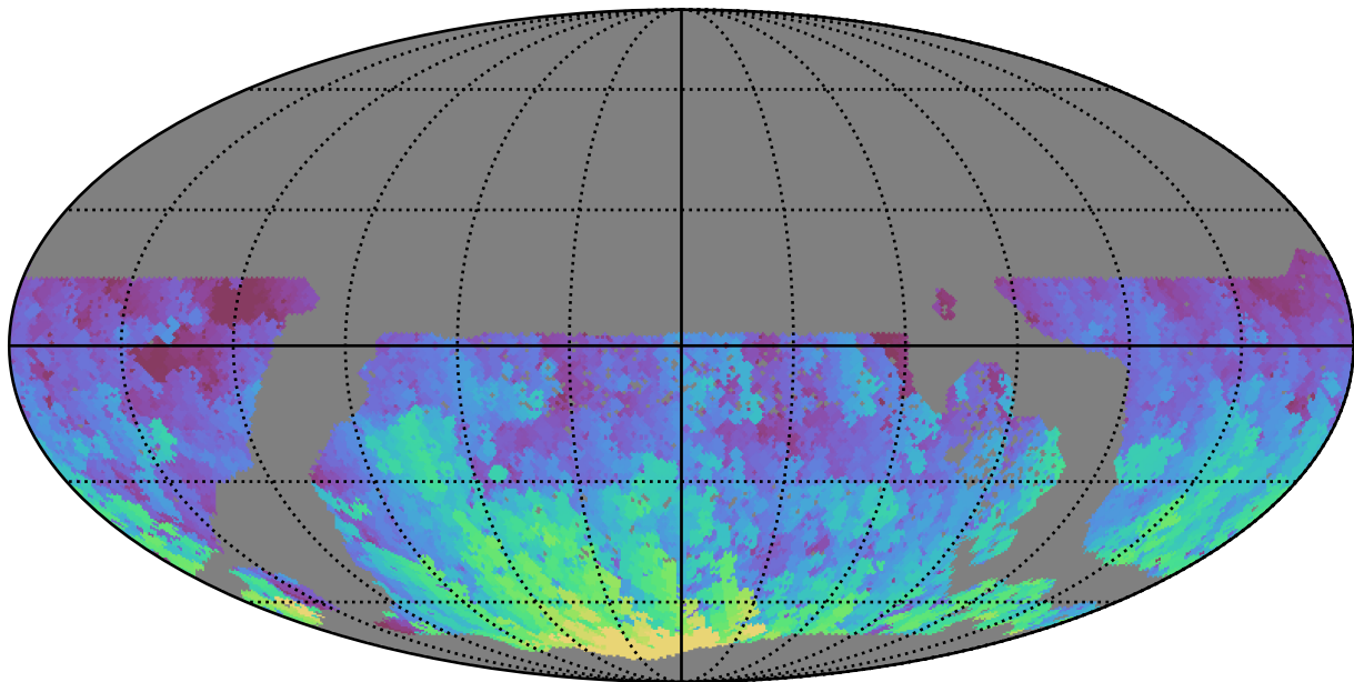
too_elab_r16_d3_gz_v3.4_10yrs WFD g band: Max HA
