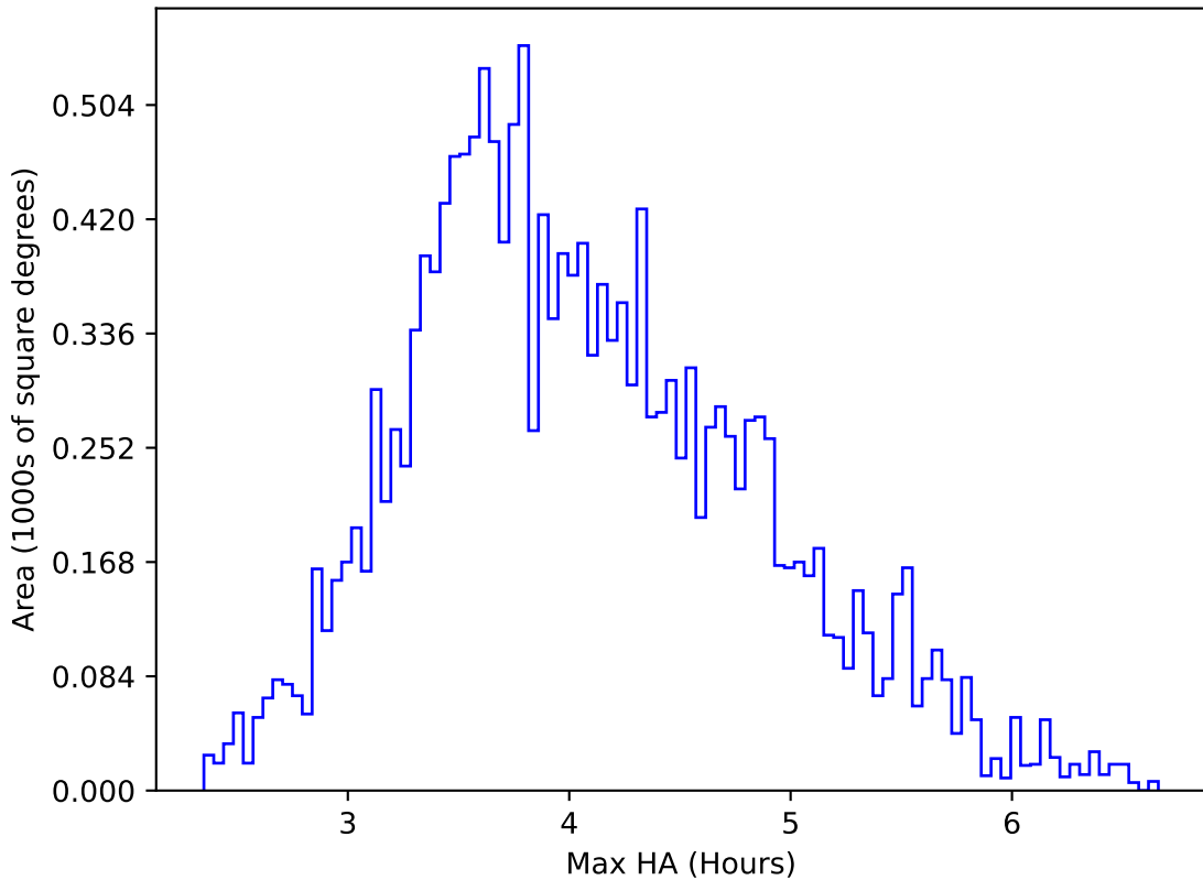
too_elab_r16_d3_gz_v3.4_10yrs WFD g band: Max HA
