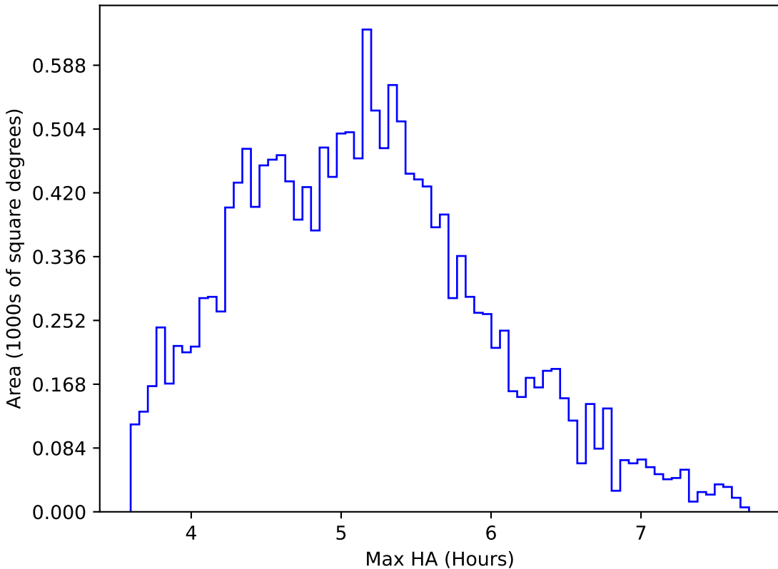
too_elab_r16_d3_gz_v3.4_10yrs WFD all bands: Max HA
