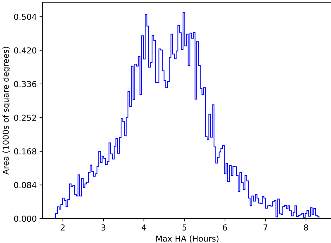
too_elab_r16_d3_gz_v3.4_10yrs All sky z band: Max HA
