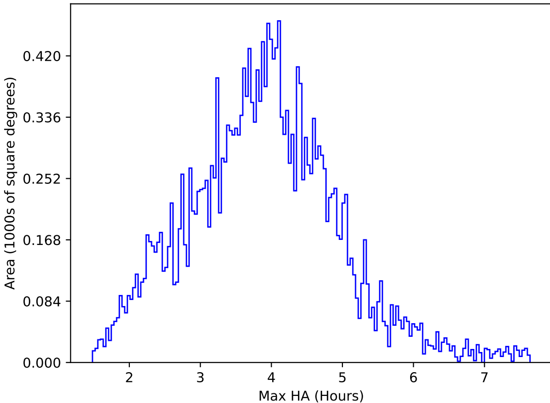
too_elab_r16_d3_gz_v3.4_10yrs All sky u band: Max HA
