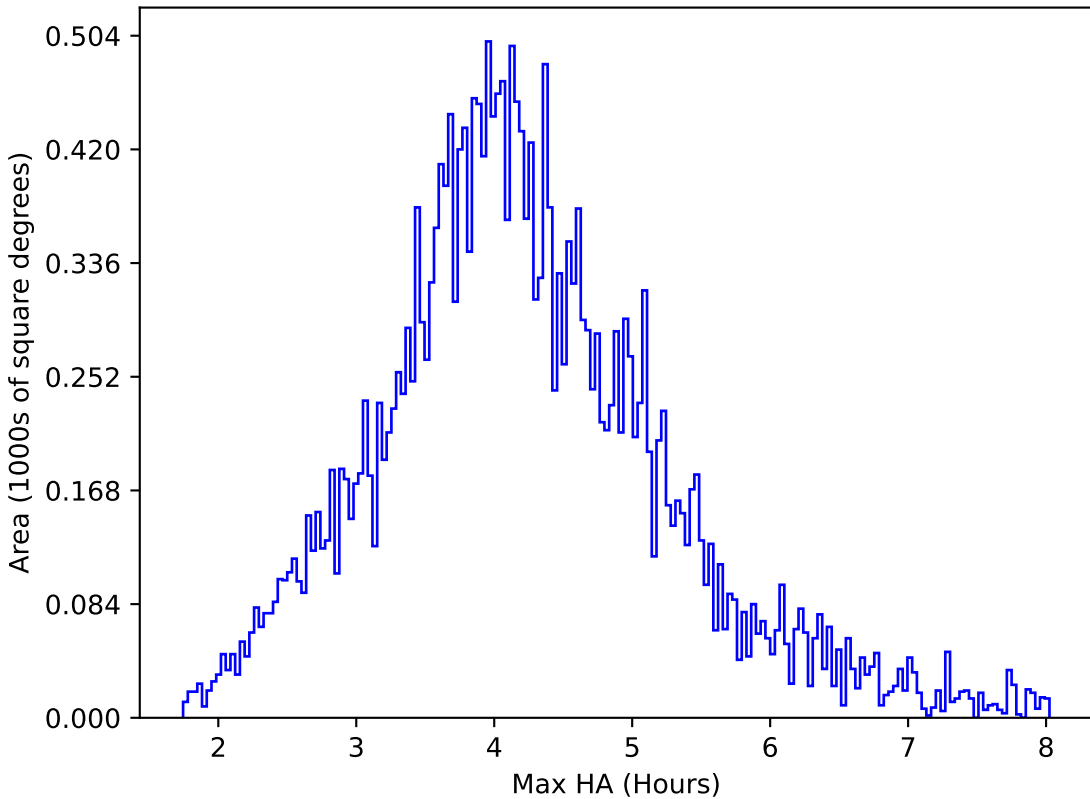
too_elab_r16_d3_gz_v3.4_10yrs All sky r band: Max HA
