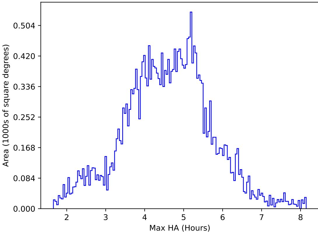
too_elab_r16_d3_gz_v3.4_10yrs All sky i band: Max HA
