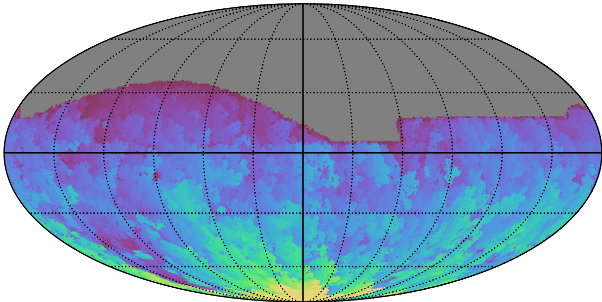
too_elab_r16_d3_gz_v3.4_10yrs All sky g band: Max HA
