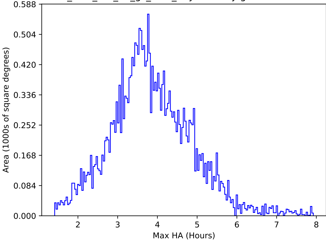
too_elab_r16_d3_gz_v3.4_10yrs All sky g band: Max HA
