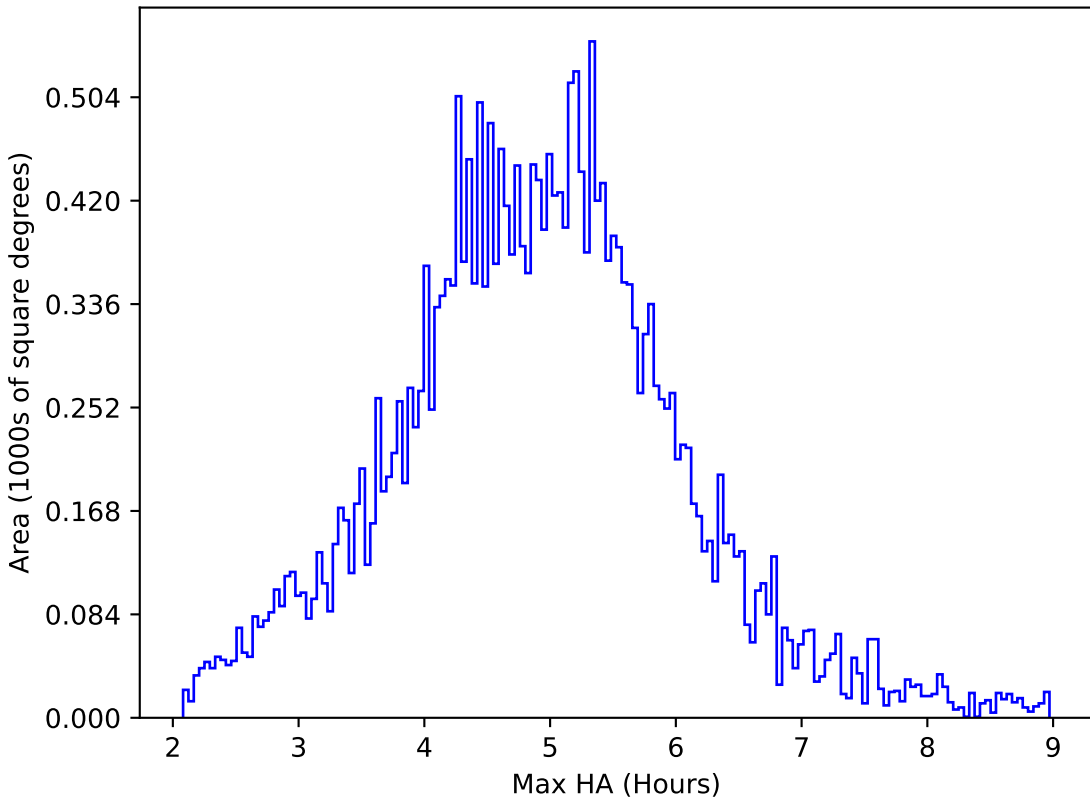
too_elab_r16_d3_gz_v3.4_10yrs All sky all bands: Max HA
