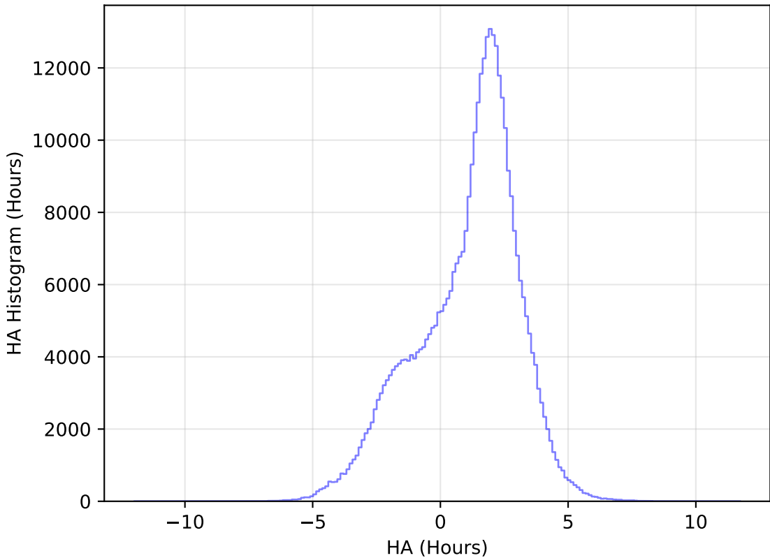
too_elab_r16_d3_gz_v3.4_10yrs WFD y band: HA Histogram
