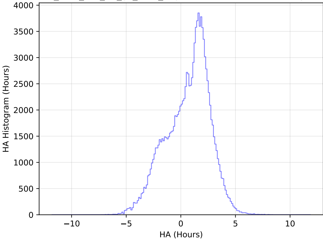
too_elab_r16_d3_gz_v3.4_10yrs WFD u band: HA Histogram
