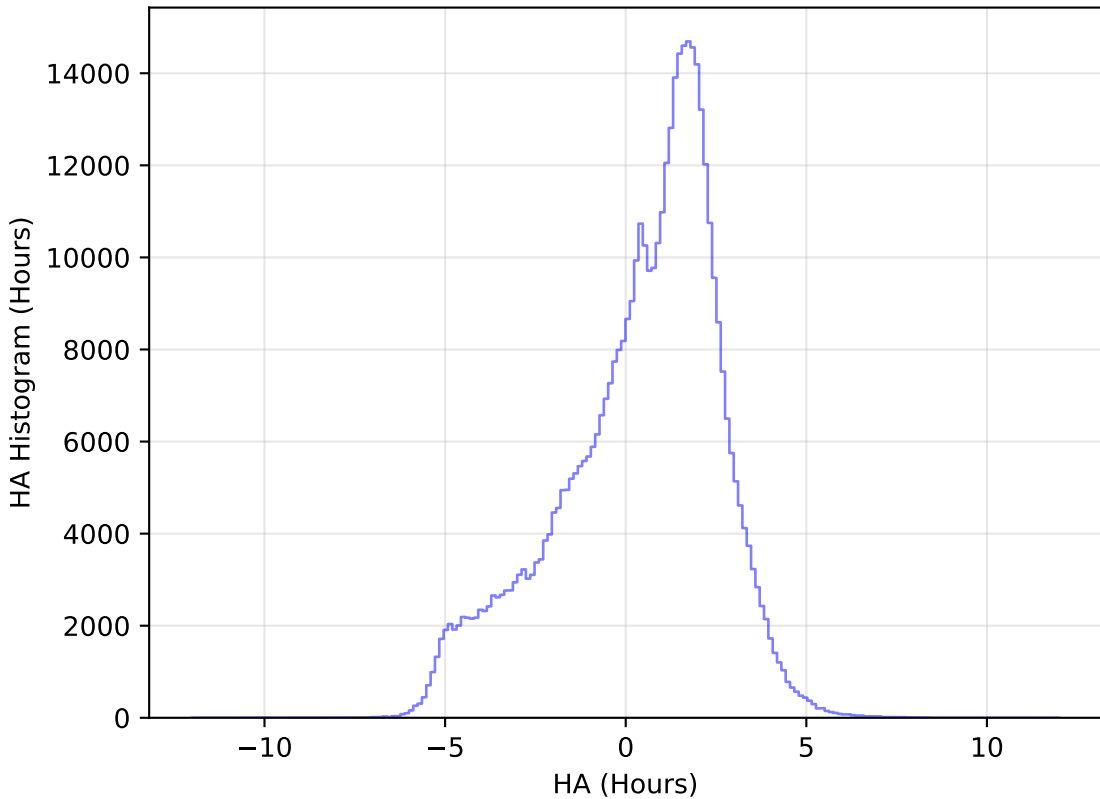
too_elab_r16_d3_gz_v3.4_10yrs WFD r band: HA Histogram
