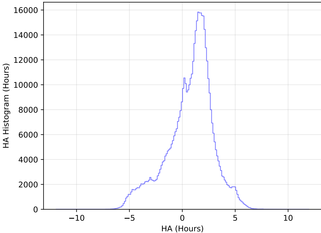
too_elab_r16_d3_gz_v3.4_10yrs WFD i band: HA Histogram
