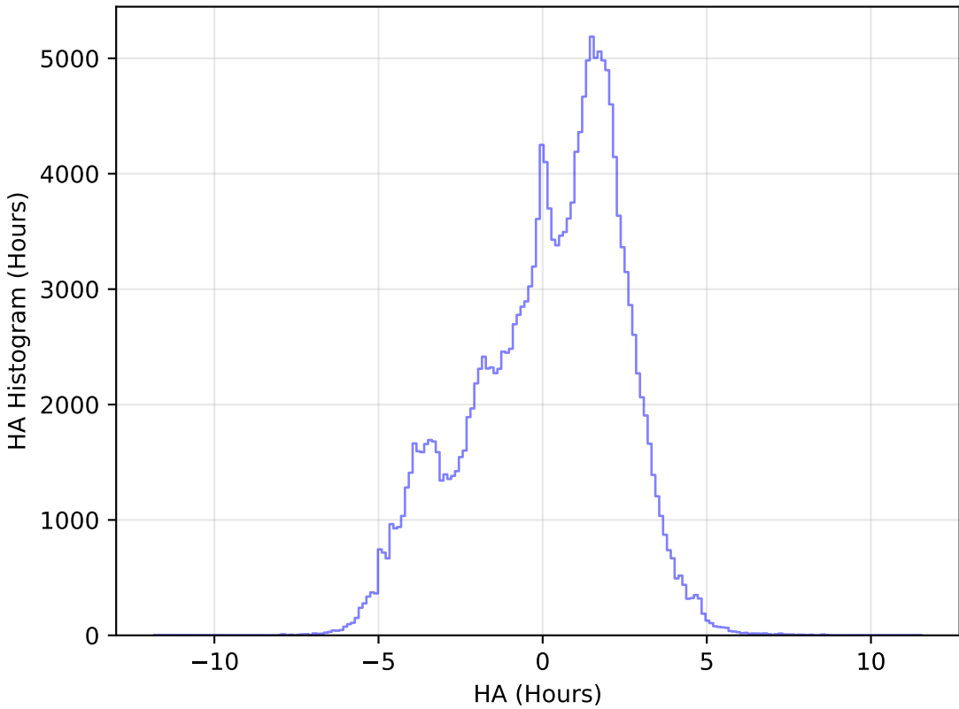
too_elab_r16_d3_gz_v3.4_10yrs WFD g band: HA Histogram
