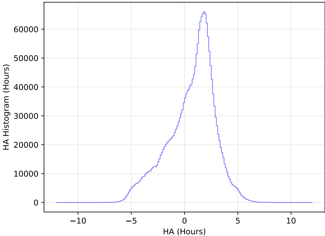
too_elab_r16_d3_gz_v3.4_10yrs WFD all bands: HA Histogram
