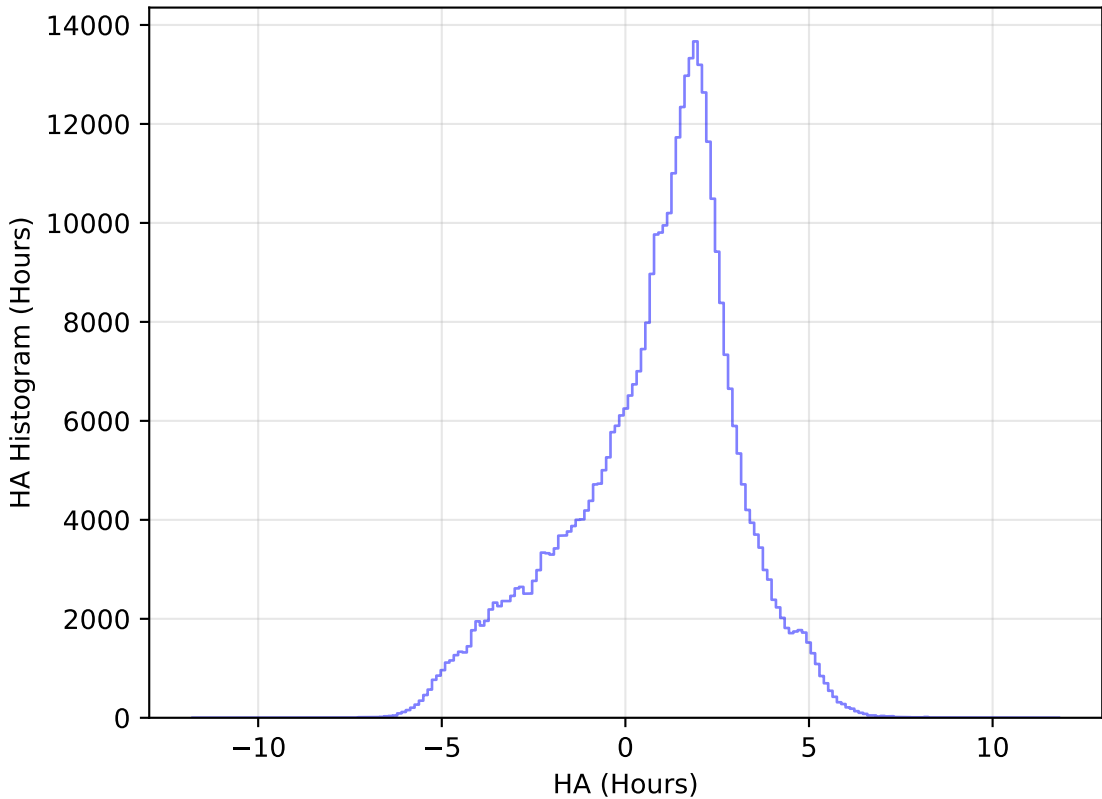
too_elab_r16_d3_gz_v3.4_10yrs All sky z band: HA Histogram
