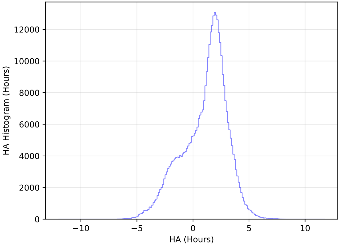
too_elab_r16_d3_gz_v3.4_10yrs All sky y band: HA Histogram
