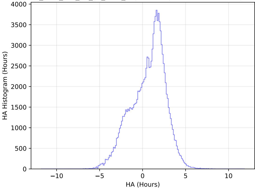
too_elab_r16_d3_gz_v3.4_10yrs All sky u band: HA Histogram
