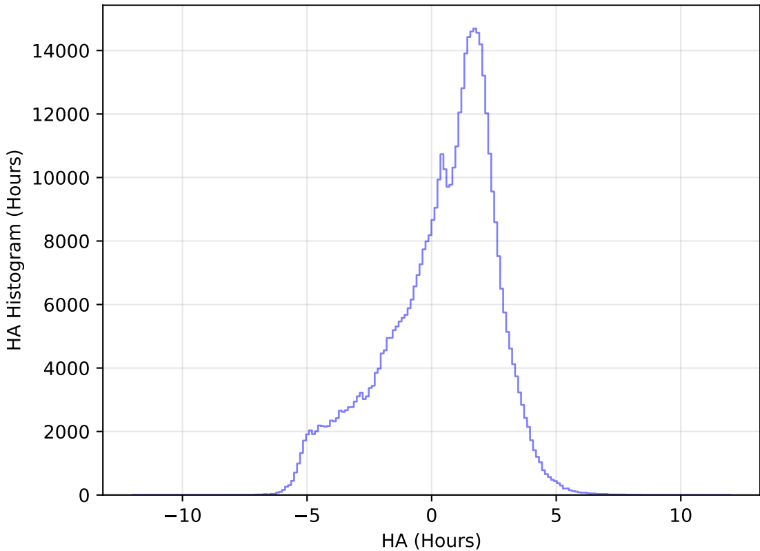
too_elab_r16_d3_gz_v3.4_10yrs All sky r band: HA Histogram
