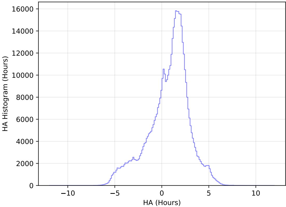
too_elab_r16_d3_gz_v3.4_10yrs All sky i band: HA Histogram
