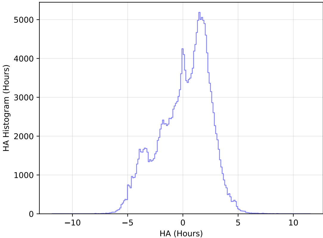
too_elab_r16_d3_gz_v3.4_10yrs All sky g band: HA Histogram
